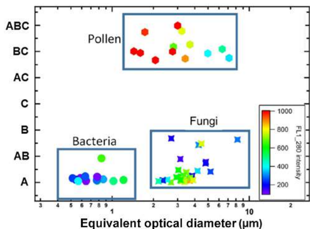
Figure 3. Assemblages of equivalent optical diameter and fluorescence type from aerosolized pure cultures of bacteria (●), fungi spores (■) and pollen grains (◆). The fluorescence type reported is a weighted composite of fluorescent type occurrence observed from each culture or pollen stock aerosolized; intensity is a relative scale.
